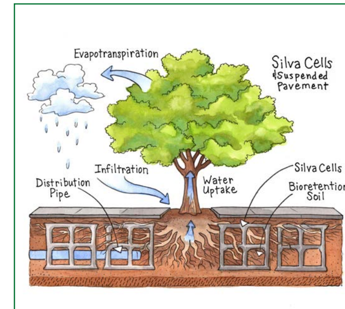
Silva Cells and Suspended Pavement
