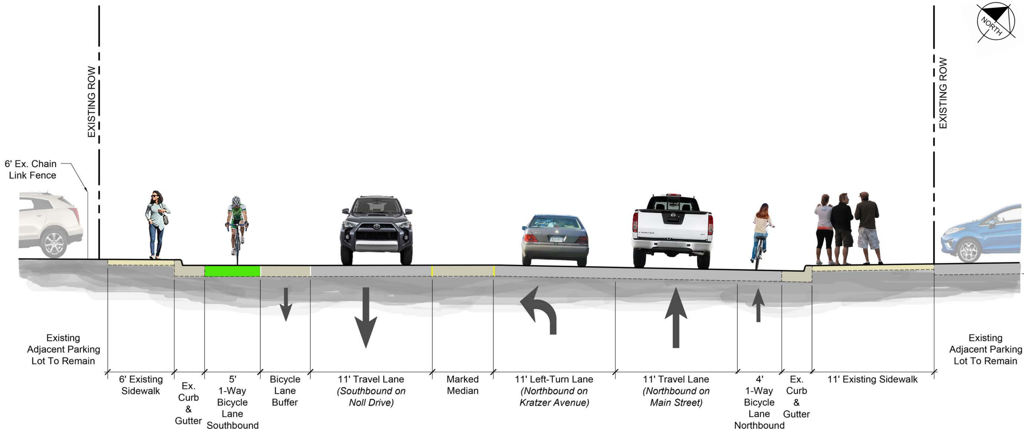
D Rendered Section on North Main Street at Main Street - Kratzer Avenue Intersection Scale: 1" = 5' - 0"
