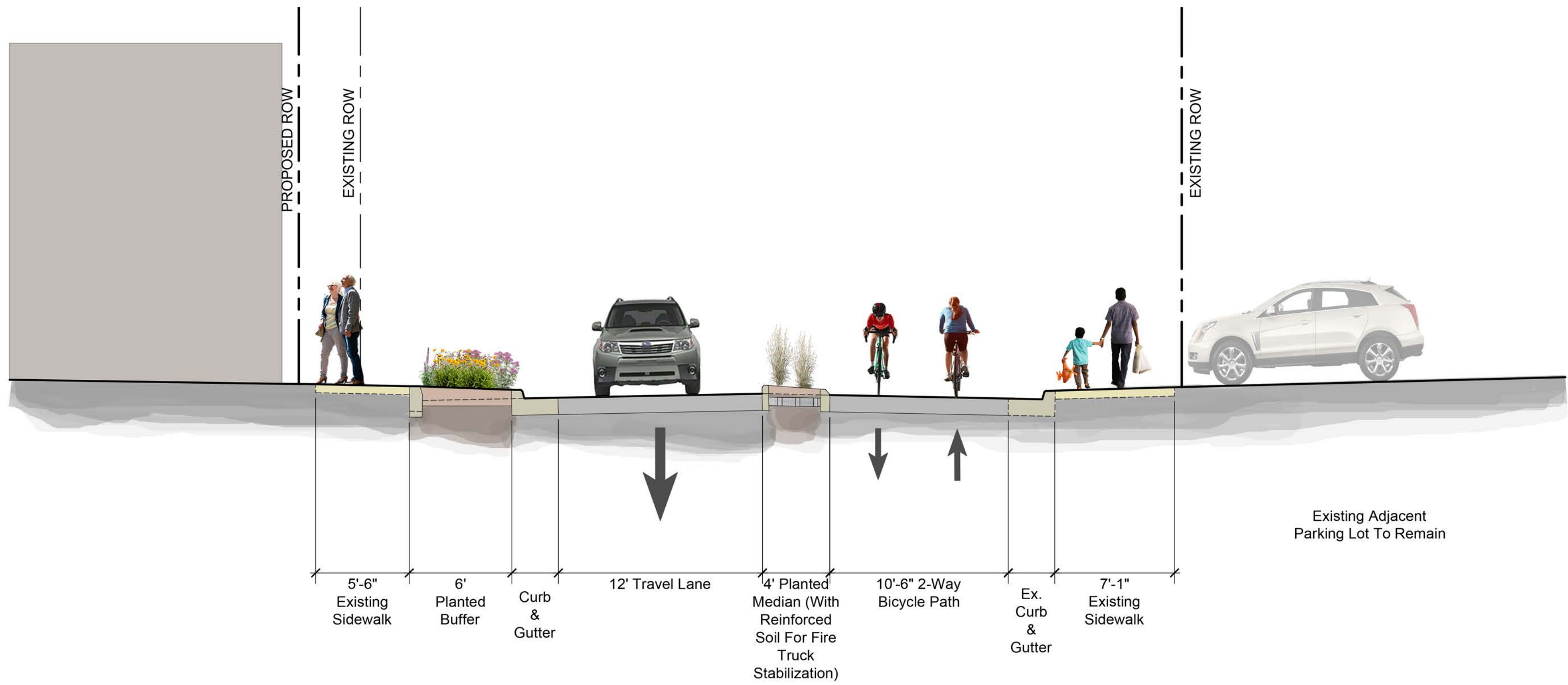
C Rendered Section on Liberty Street Near Elizabeth Street Scale: 1" = 5' - 0"
