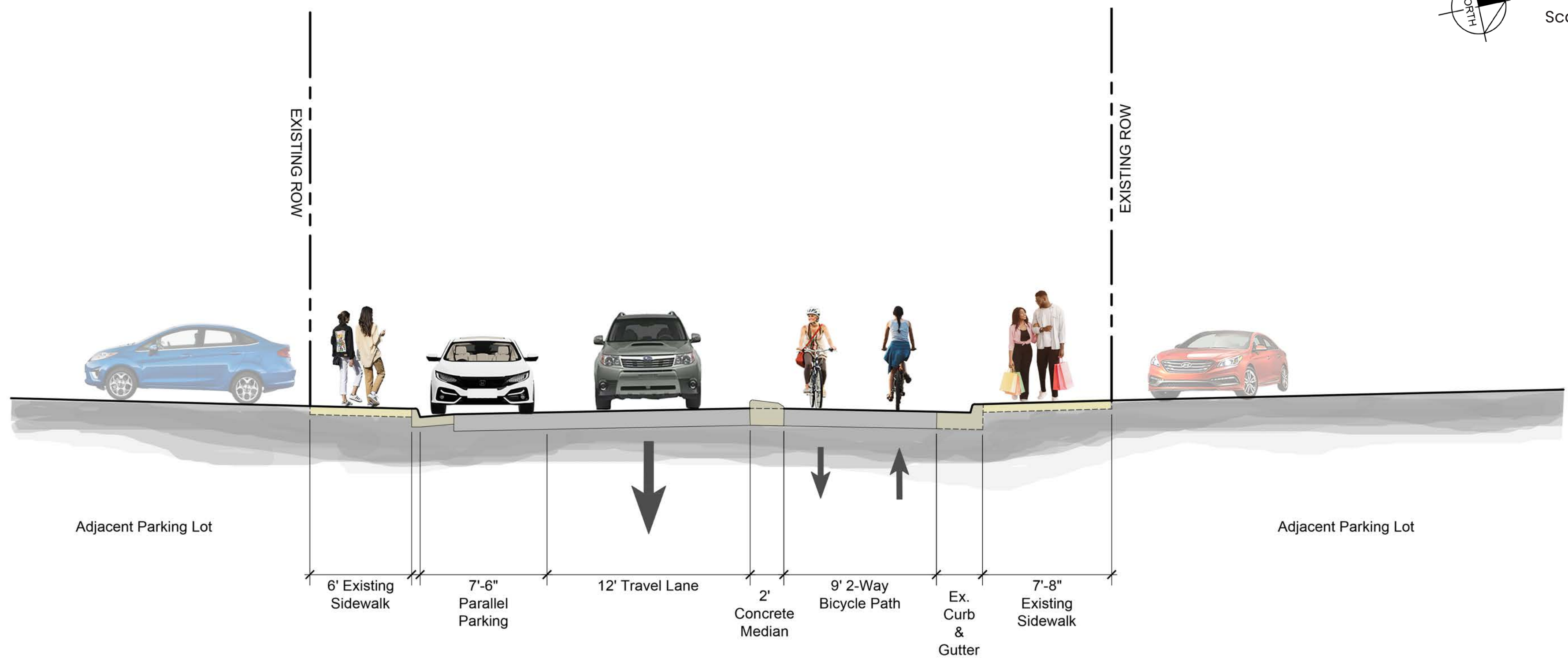
B Rendered Section on Liberty Street Near Market Street Scale: 1" = 5' - 0"
