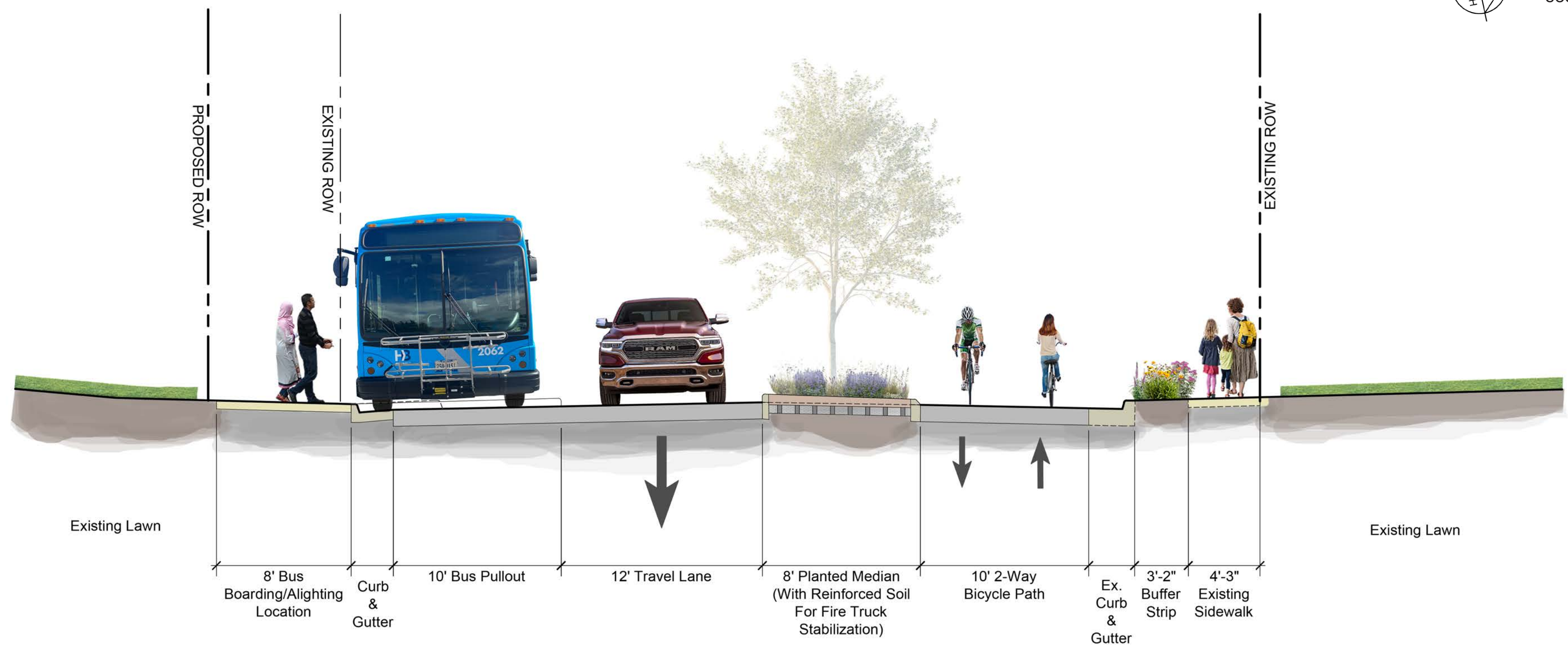
A Rendered Section on Liberty Street Near Grattan Street Scale: 1" = 5' - 0"
