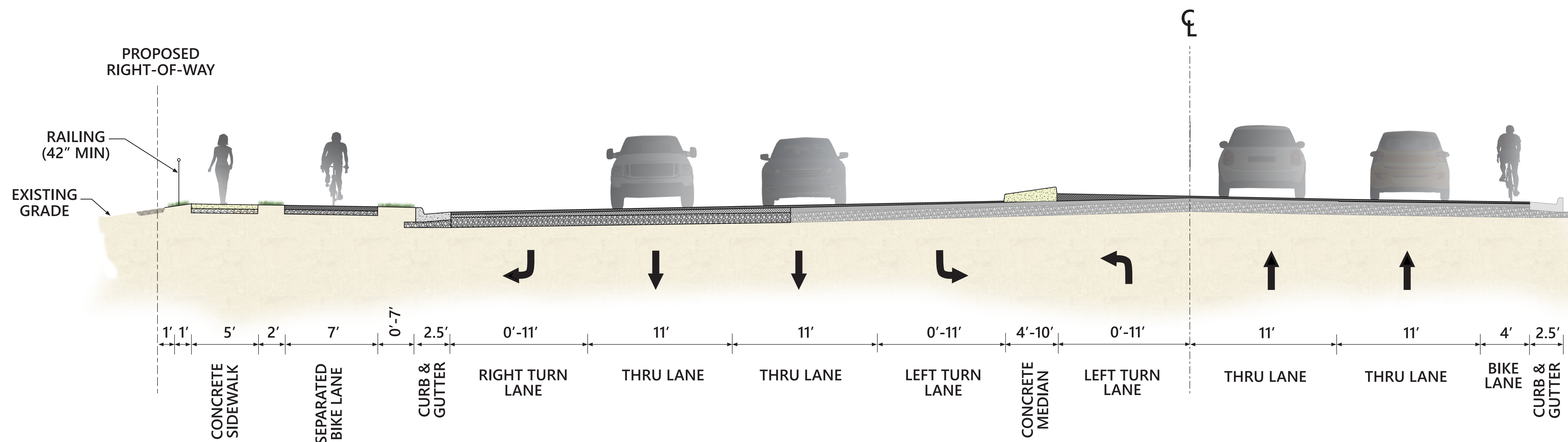
TYPICAL SECTION PORT REPUBLIC ROAD @ BRADLEY DRIVE
