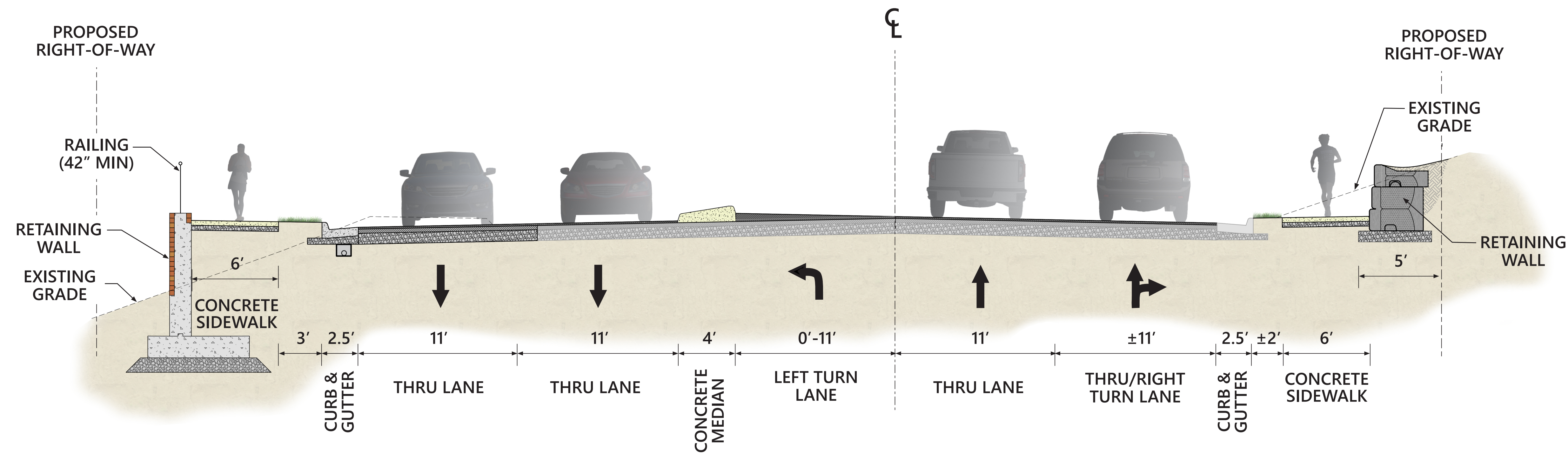
TYPICAL SECTION PORT REPUBLIC ROAD @ BLUESTONE DRIVE
